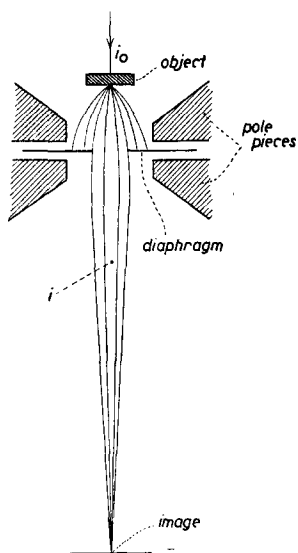
Fig. 1. Simplified scheme of the electron beam in the electron microscope.
