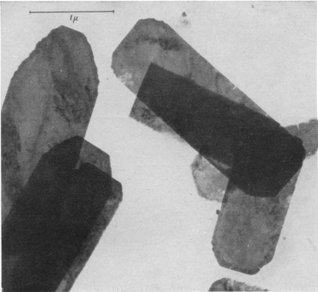
Fig. 3. \text{WO}_3 crystals. 100 kV.
